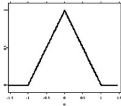
Triangular
